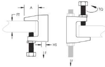
Universal beam clamp for standard beams
